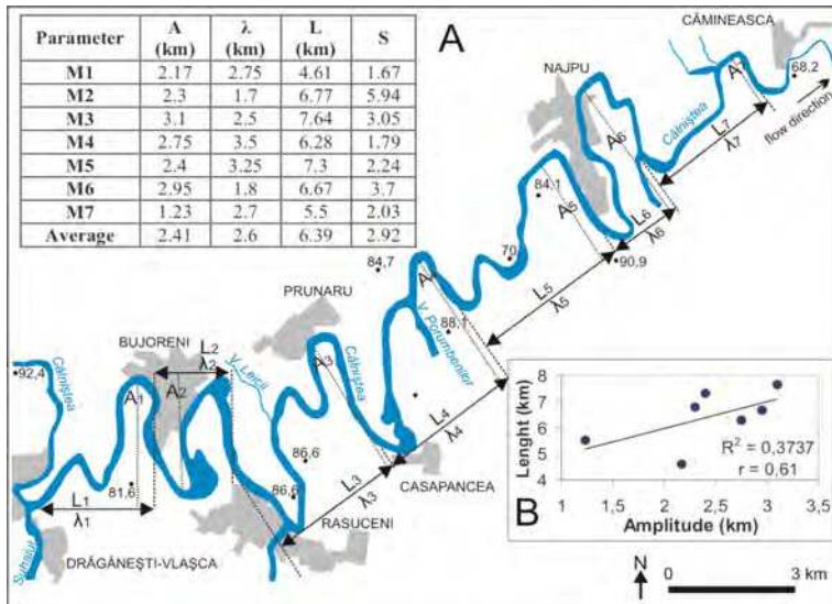
Fig. 11A. The meander morphometry of the Câlniștea River (according to Grecu et al., 2010b, modified). B. Corellation between the length and the amplitude of the meanders of the Câlniștea River in the study reach. M1...M7: meander number; A: meander amplitude; \lambda : meander wavelength; L: channel length; S: sinuosity ratio.
