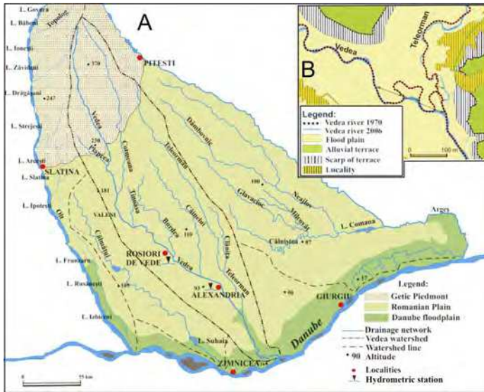
Fig. 10A. The central sector of the Romanian Plain, and the location of the Vedeia and Câlniștea rivers. B. The lateral dynamics of the Vedeia channel near the junction of the Teleorman between 1970 and 2006 (according to Grecu et al., 2010c, modified). The arrows in B show the most modified sectors.
